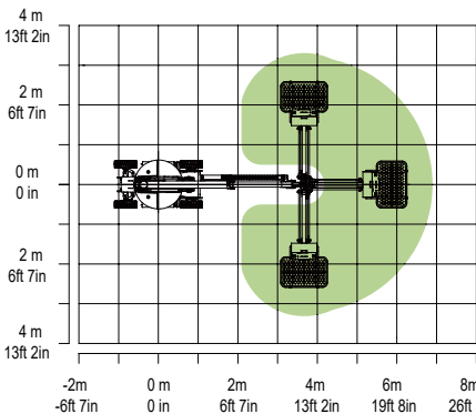
Range of Jib Swing Motion ZA10RJE
