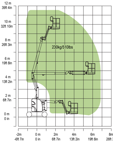
Range of Motion ZA10RJE
